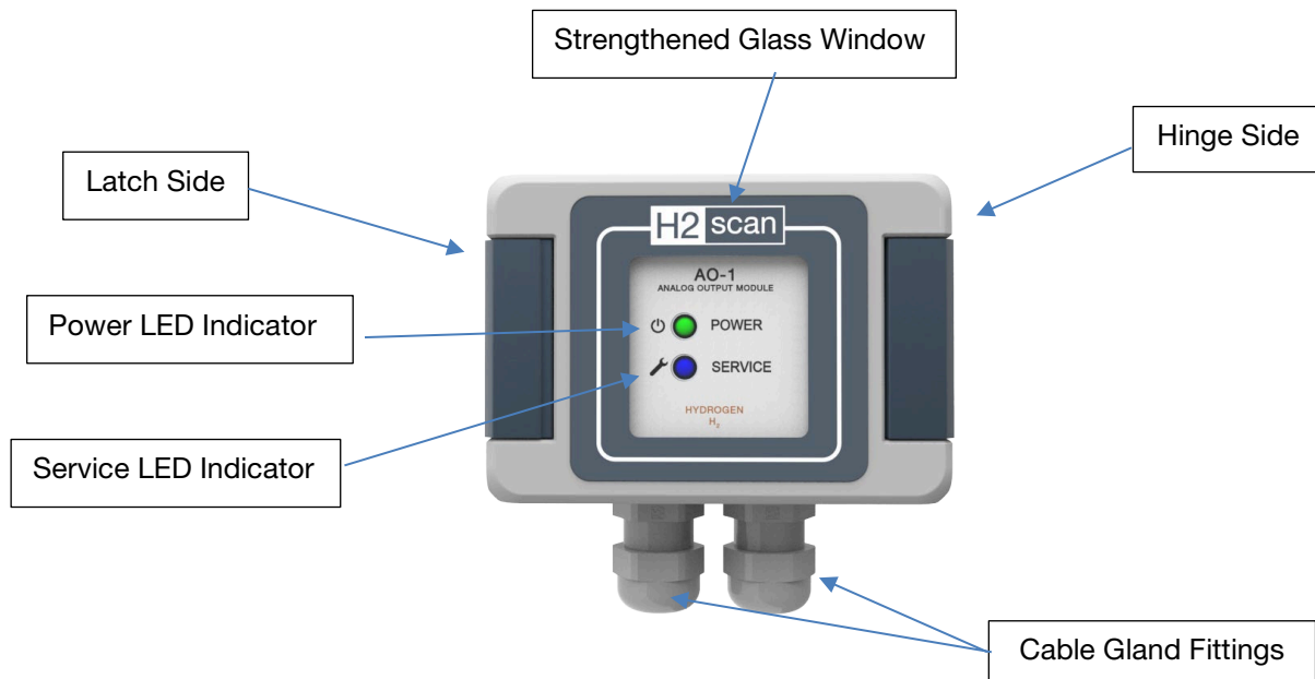
Figure 2: GSAO-1 Front View Features
