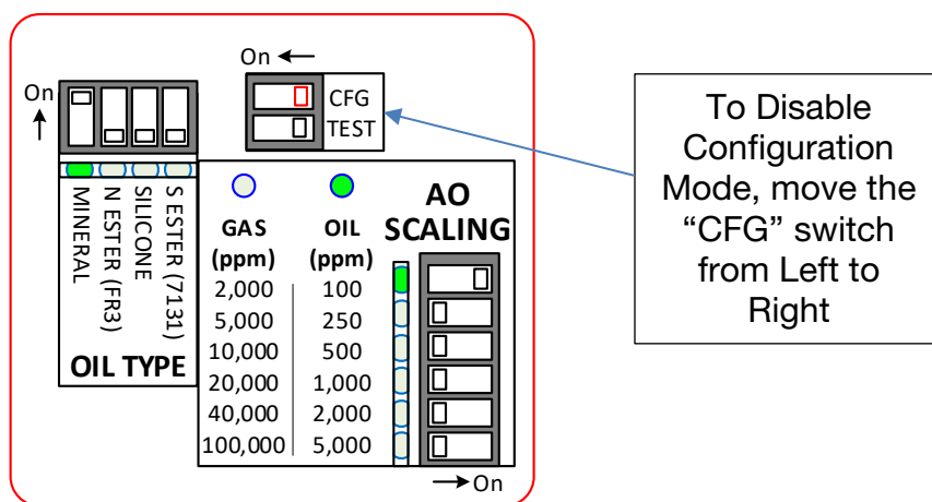
Figure 23: Disabling Configuration Mode
