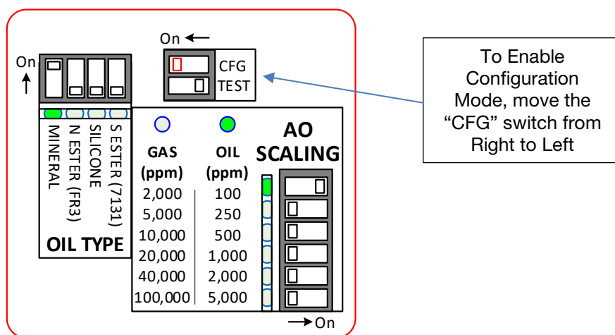
Figure 19: Enabling Configuration Mode
