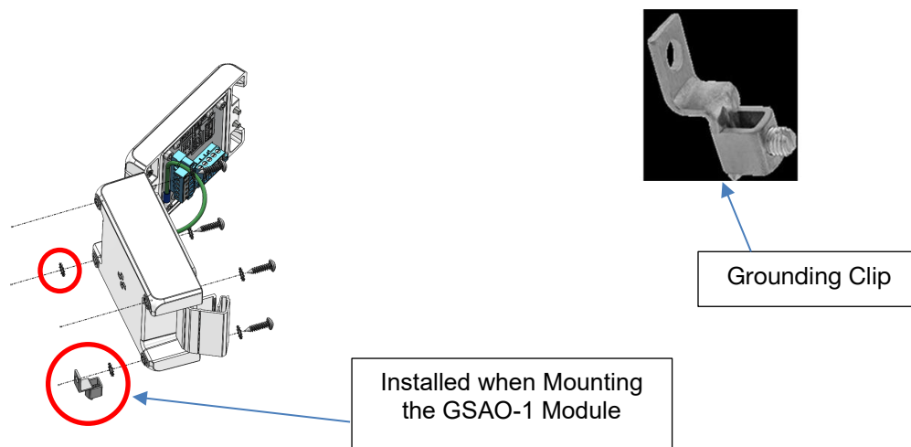
Figure 7: GSAO-1 External Grounding Solution
