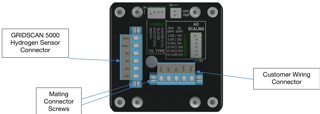
Figure 8: GSAO-1 Electrical Connectors
