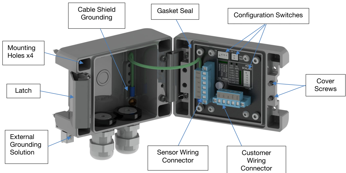
Figure 3: GSAO-1 Open View Features
