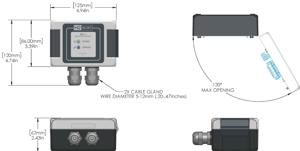
Figure 1: GSAO-1 Dimensions
