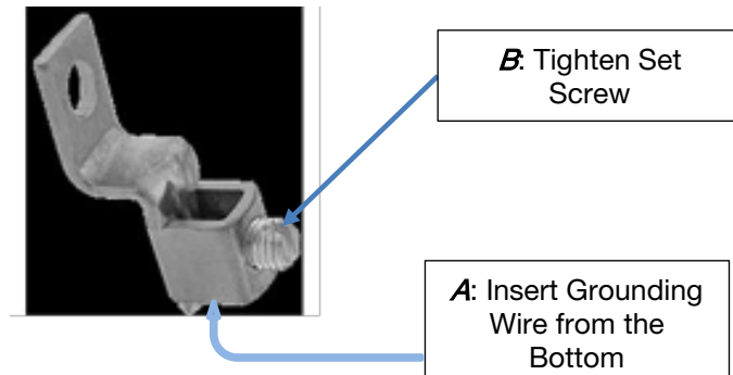
Figure 9: GSAO-1 External Grounding Connector
