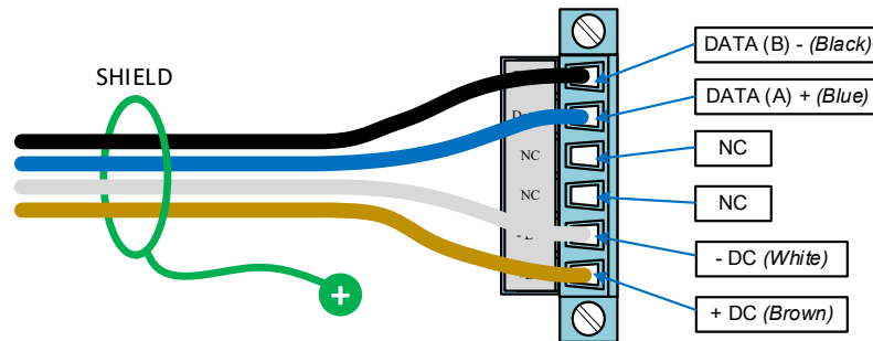
Figure 12: GRIDSCAN 5000 Hydrogen Sensor Connector with Wires
