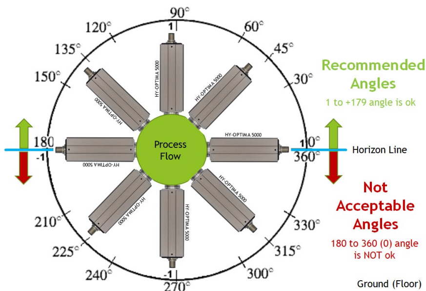
Figure 3: Acceptable and Unacceptable Mounting Orientations
