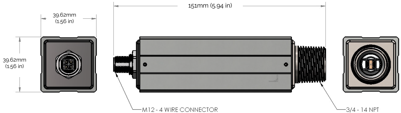
Figure 1: HY-OPTIMA 5030 Series Hydrogen Sensor Dimensions
