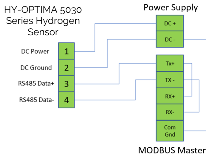
Figure 2: Connection to Modbus RTU Master
