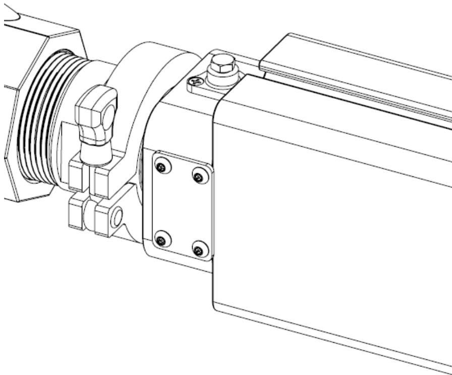
Figure 6: Clamp Installation
